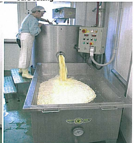
Curd discharge
